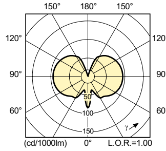
LDLD_CDM-T-E_0011-Light distribution diagram
