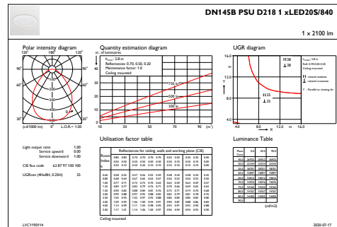
IFGU1_DN145BPSUD2181xLED20S840
