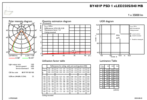
IFGU1_BY481PPSD1xLED350S840MB
