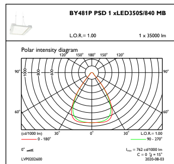
OFPC1_BY481PPSD1xLED350S840MB
